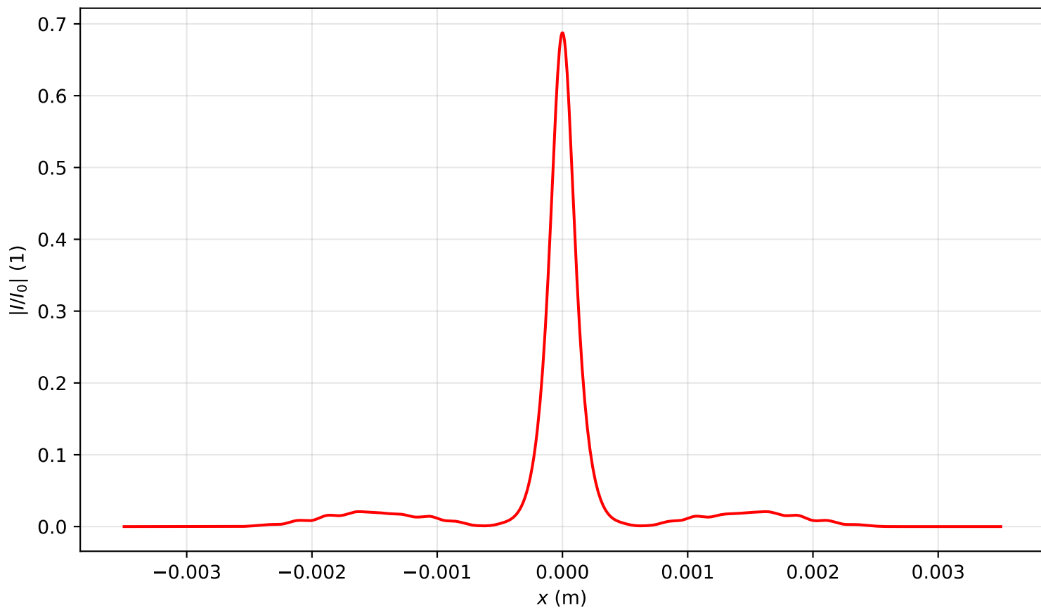
Intensity profile I(x, y = 0, z = 1.592)/I_0 , P_{in}=9.0P_{cr} , artificial time
